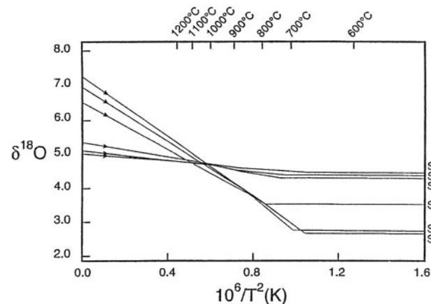
Figure 11. Isotope Exchange Trajectories (IET) for magnetite from six rocks from the Sybille Fe-Ti-oxide quarry, Laramie anorthosite complex. The average temperature of intersection, 1077 \pm 25^\circ\text{C} , is higher than T_C for any mineral in these rocks, and it is interpreted as the solidus temperature of the magma (from Farquhar et al. 1993).
