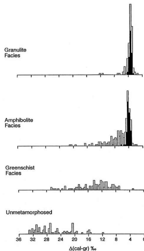
Figure 17. Carbon isotope fractionations as a function of metamorphic grade. (A, left) Compilation of measured values of \Delta(\text{Cc-Gr}) shows scatter and disequilibrium at greenschist facies and lower temperature conditions. Many amphibolite facies and most granulite facies samples show a tight clustering of values consistent with isotope equilibration above 600°C. Values in black are from the Adirondacks (from Kitchen and Valley 1995). (B, below) Values of \delta^{13}\text{C} for a Liassic black shale formation (Hoefs and Frey 1976) showing successive approach to equilibrium at maximum T = 500\text{--}600^\circ\text{C} (from Sharp et al. 1995).
