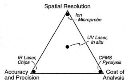
Figure 1. Advantages and trade-offs of new analytical techniques for stable isotope analysis (see Table 1). At present, the best accuracy and precision is achieved for \delta^{18}\text{O} by IR-laser fluorination of chips or powdered samples; the fastest and least expensive analyses are made by automated pyrolysis systems with continuous flow mass-spectrometers (CFMS); and the smallest samples and best in situ spatial resolution is attained by ion microprobe. The capabilities of in situ UV-laser fluorination are intermediate.
