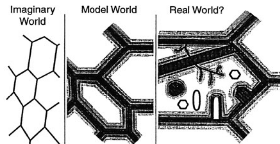
Figure 12. Cartoons of minerals showing gradients of isotope ratio due to exchange in shades of gray. (A) the "imaginary world" where all minerals are homogeneous and equilibrated, and there are no gradients. (B) the idealized "model world" where exchange takes place radially inward from grain boundaries by diffusion. Actual gradients would be smooth. (C) the "real world" will show effects of diffusion and may also have fast pathways of exchange due to recrystallization, micro-cracks, dislocations, inclusions or deformation.
