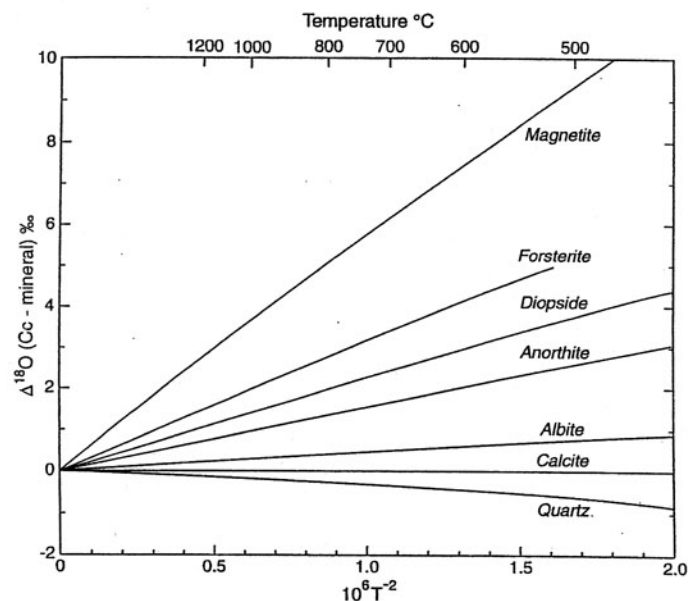
Figure 2. Experimentally determined oxygen isotope fractionations between calcite and quartz, albite, anorthite, diopside, forsterite and magnetite (Clayton and Kieffer 1991).
