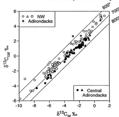
Figure 19. Carbon isotope thermometry for Adirondack marbles. (A, left) Plot of \delta^{13}\text{C}(\text{calcite}) vs. \delta^{13}\text{C}(\text{graphite}) . Open symbols are for upper the amphibolite facies NW Adirondacks and closed symbols are for the granulite facies Adirondack Highlands. (B, below) Values of \Delta(\text{Cc-Gr}) in per mil and resulting isopleths for 675^\circ\text{C} parallel the strike of the terrane and, show lower metamorphic temperatures centered on Gouverneur and increasing towards granulite facies rocks to the SE and to NW. Note outcrop tests at Fish Creek (FC), the Train Wreck (TW) and the Valentine Mine (VM) (from Kitchen and Valley 1995).
