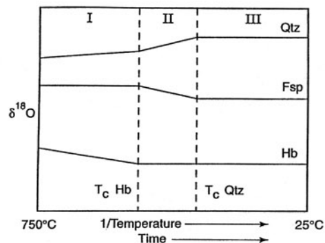
Figure 8. Schematic representation of \delta^{18}\text{O} of quartz, feldspar and hornblende in an idealized granite undergoing diffusive exchange while cooling as described by the model of Gilotti (1986). At high temperatures, above T_c(\text{Hb}) , all three minerals are open to exchange and maintain equilibrium (Period I). At lower temperatures (Period II) hornblende is "closed" to oxygen diffusion and only quartz and feldspar continue to equilibrate. In this period, \Delta(\text{Fsp-Hb}) decreases although no feldspar-hornblende exchange occurs. Finally, below T_c(\text{Qtz}) , no further exchange can take place (Period III) and final fractionations are preserved (from Eiler et al. 1992).
