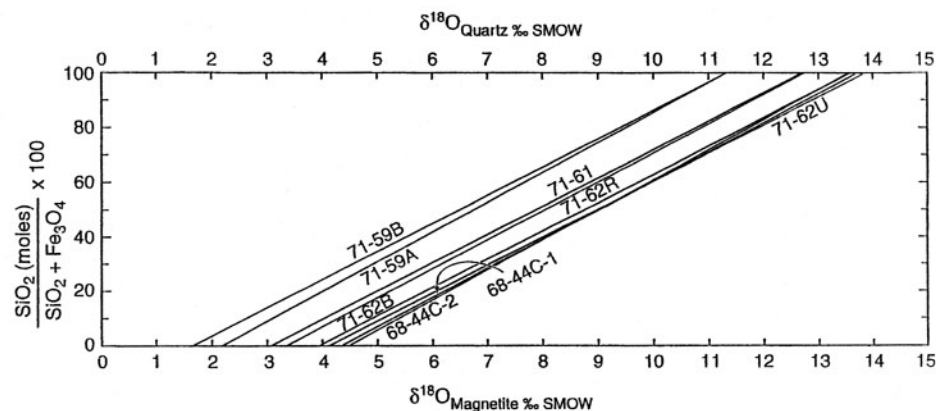
Figure 14. Plot of \delta^{18}\text{O}(\text{magnetite}) vs. \delta^{18}\text{O}(\text{quartz}) for amphibolite facies quartzites from Black Mtn., New Hampshire. The nearly parallel tie-lines indicate that fractionations are self-consistent for these eight samples from one outcrop. The average oxygen isotope temperature of 542°C is in excellent agreement with that from petrology (530°C). (from Rumble (1978)).
