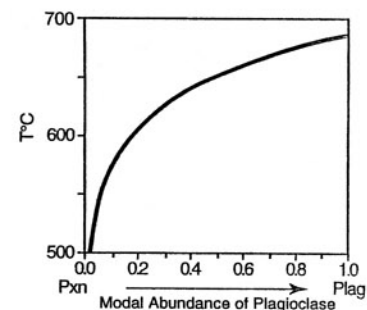
Figure 9. Plot of apparent temperature recorded between a mineral with slow oxygen diffusion (pyroxene) and a mineral with fast diffusion (plagioclase) vs. the modal percentage of plagioclase in a bi-mineral rock. Cooling is at 5^\circ\text{C/m.y.} after peak equilibration at 750^\circ\text{C} . In feldspar dominated rocks, T_A may preserve peak temperature, but for a rock dominated by pyroxene, T_A can be hundreds of degrees below peak T approaching 250^\circ\text{C} , T_c(\text{plag}) . The mode effect is modeled by the Fast Grain Boundary diffusion model and predicts that refractory accessory mineral (RAM) thermometers are most reliable (from Eiler et al. 1993).
