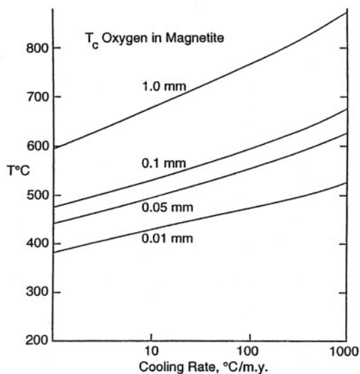
Figure 6. Calculated values of closure temperature for oxygen diffusion in magnetite of 1 to 0.01 mm in radius at cooling rates of 1 to 1000°C/m.y. (Gilotti and Hess 1988).
